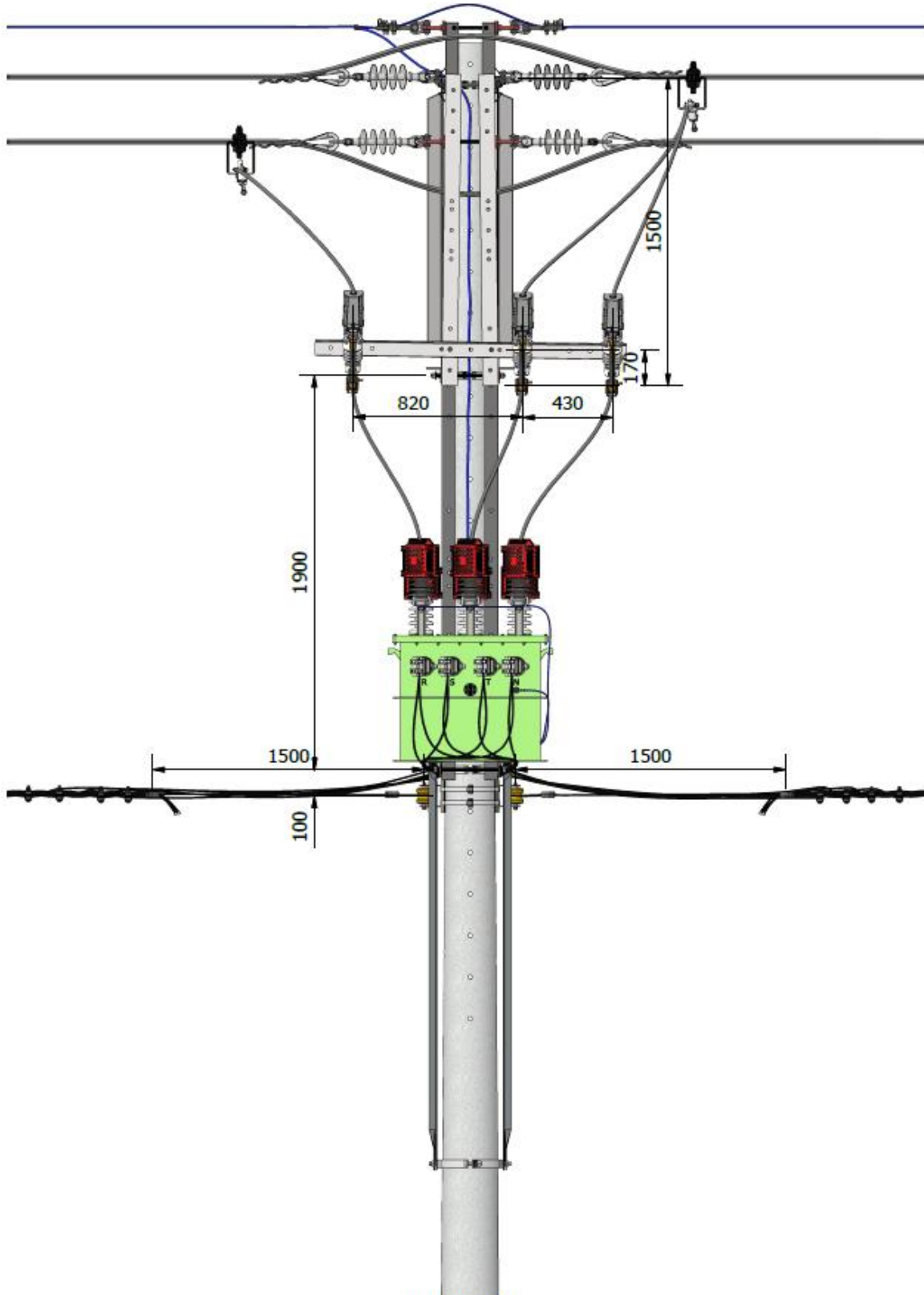
Vista frontal
