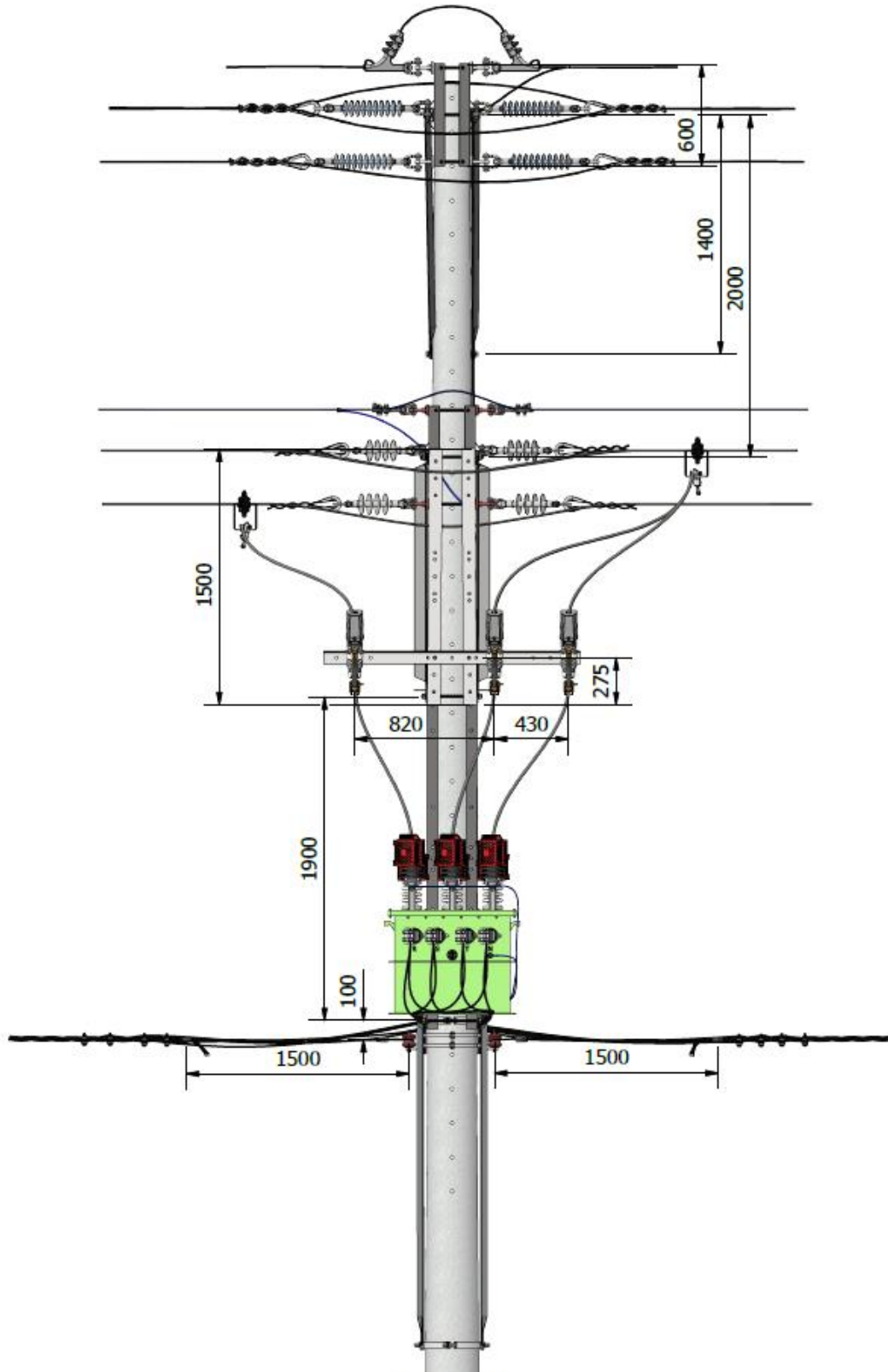
Vista frontal
